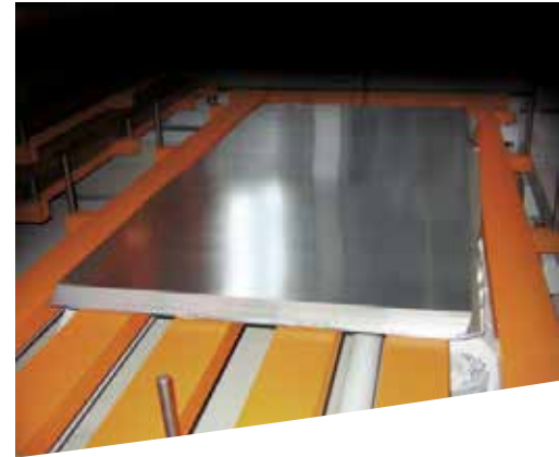
System pallet for loading sheet metal packs of different sizes with a carrying capacity of 3 to (1,5 x 3 m), six floor bars.
